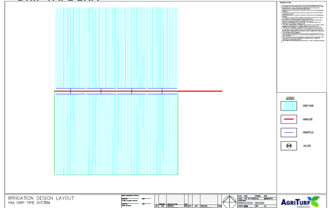
DRIP TAPE 1HA
